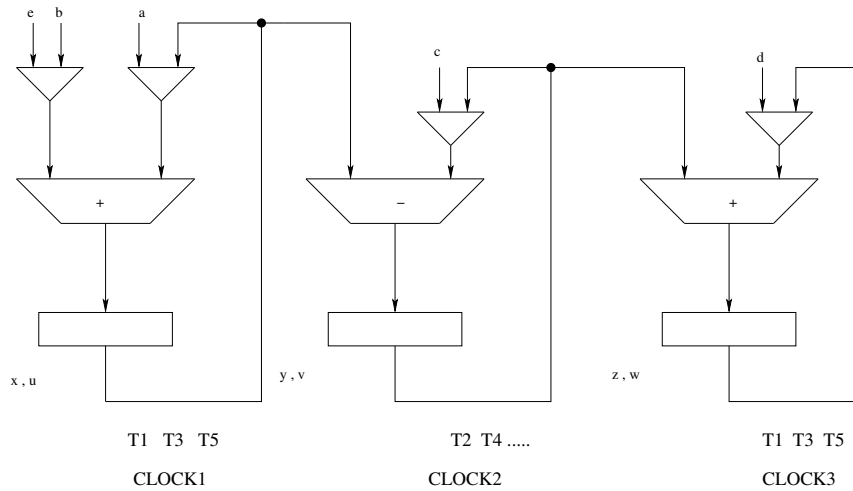
Figure 2.13. Partitioned Circuit
