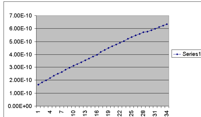
Figure 3.12. Leakage Power Vs Transistor Width
